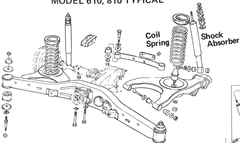
MODEL 610, 810 TYPICAL
