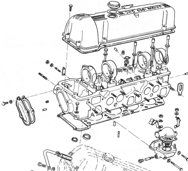
Cylinder Head
