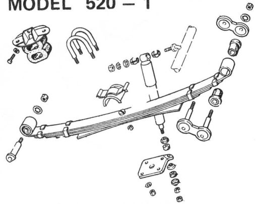
MODEL 520 - 1
