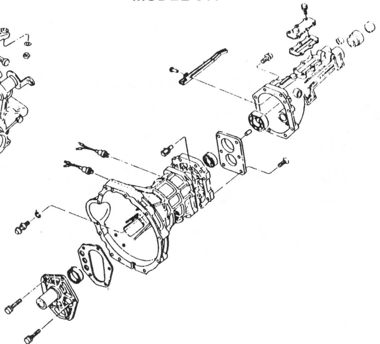
MODEL 810
